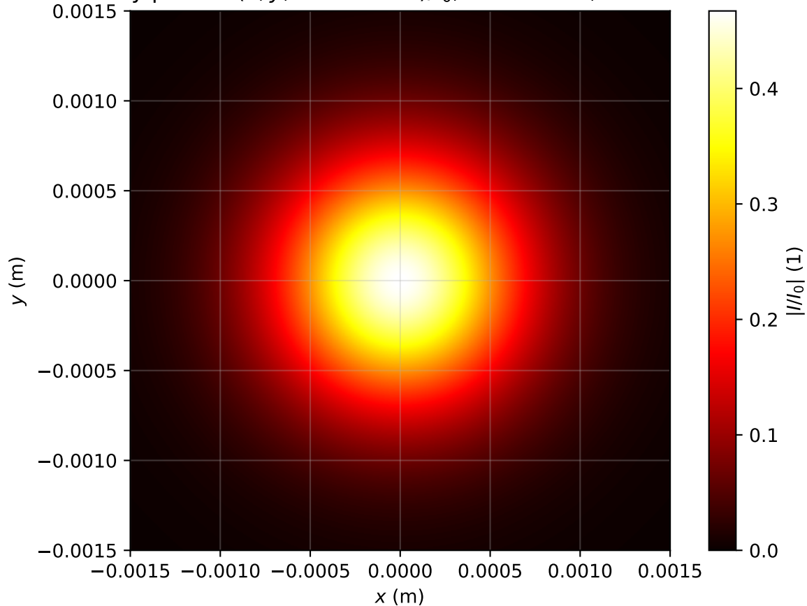
Intensity profile I(x, y, z = 3.503m)/I_0 , Pin=0.5Pcr, artificial time
